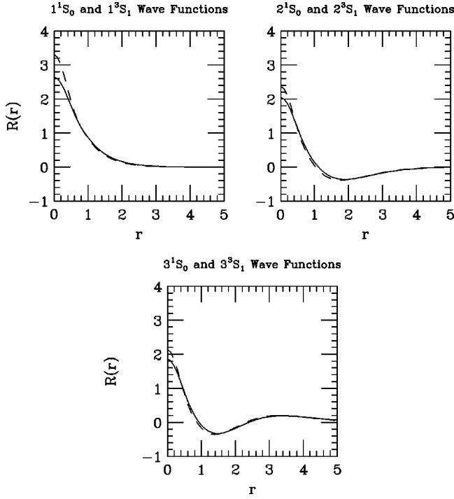
FIG. 1. Comparison of spin-singlet (dashed) and spin-triplet (solid) wave functions for nSb\bar{b} levels.
